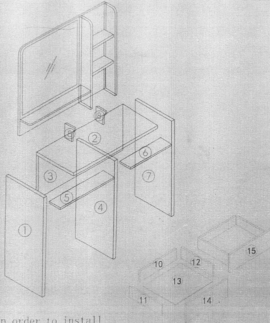
dresser Sequential installation diagram
